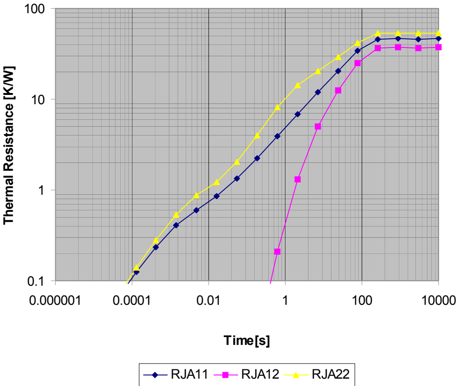
Figure 20. Transient Thermal 1W Step Response; Device on 1s JEDEC Standard Thermal Test Board with Heat Spreading Areas 600 Sq. mm
