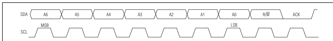
Figure 6. Slave Address
