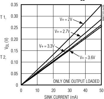
SINK CURRENT vs. V_{OL}
