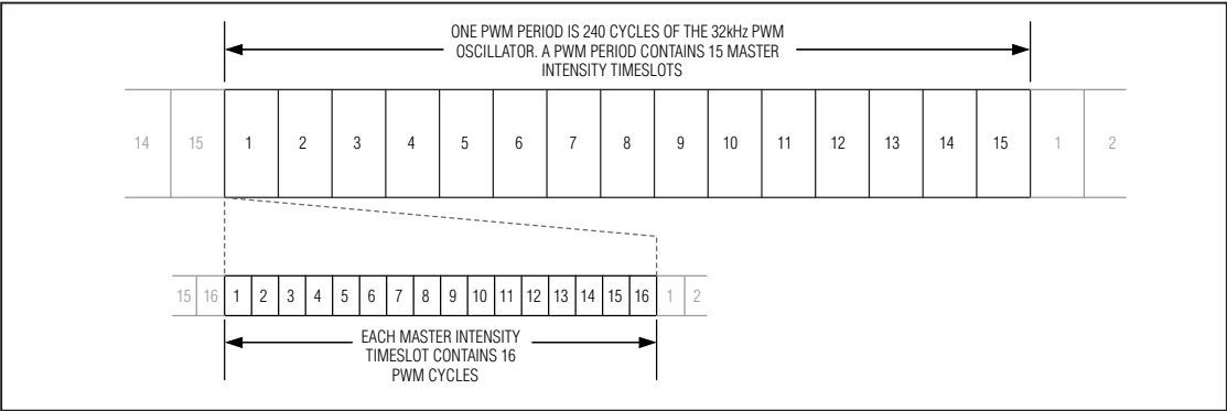
Figure 11. PWM Timing
