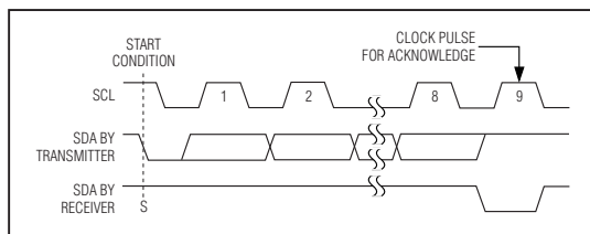
Figure 5. Acknowledge
