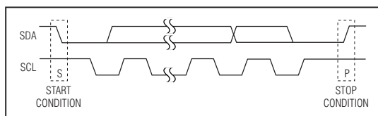
Figure 3. Start and Stop Conditions
