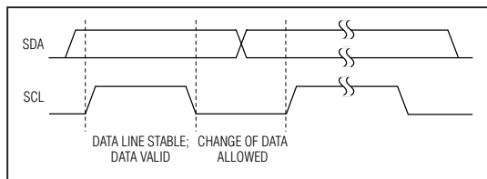
Figure 4. Bit Transfer
