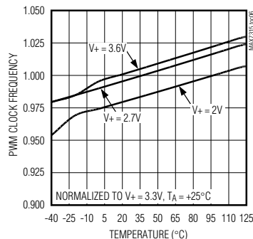
PWM CLOCK FREQUENCY vs. TEMPERATURE
