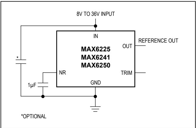
Figure 2. Noise-Reduction Capacitor
