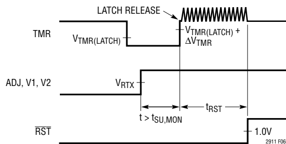
Figure 6b. Input Toggled High While Timer Latched. RST Goes High t_{RST} After Latch Release
