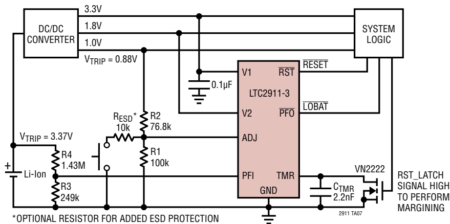
Triple Supply Monitor with Early Power-Fail Warning (With Manual Reset and Latchable Reset for Margining)
