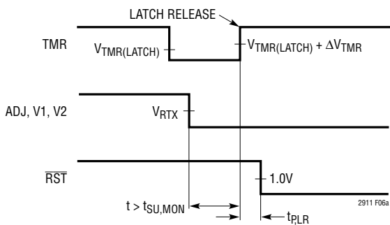
Figure 6a. Input Toggled Low While Timer Latched. RST Goes Low t_{PIR} After Latch Release
