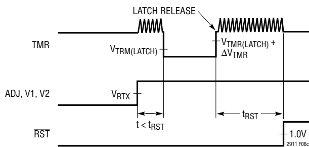
Figure 6c. Timer Latched Before Timeout. After Latch Release, RST Stays Low for a Full Timeout Before Going High
