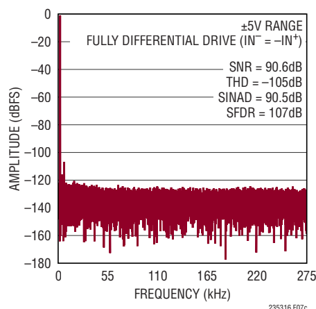
Figure 7c. IN+/IN- = 450mV 200Hz Fully Differential Sine, 0V ≤ V CM ≤ 24V, 32k Point FFT, f SAMPL = 550ksps. Circuit Shown in Figure 7a
