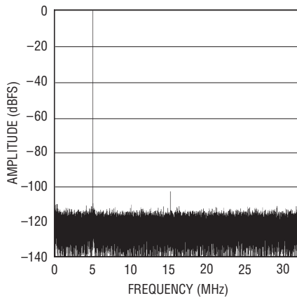
LTC2205: 64K Point FFT, 65\text{Mps} , f_{IN} = 5.1\text{MHz} , -1\text{dBFS} , \text{PGA} = 1 , \text{DITH} = 0
