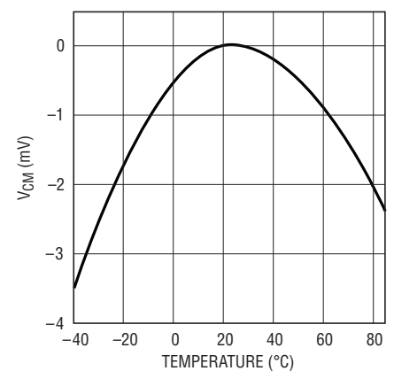
LTC2205: V_{CM} Drift vs Temperature
