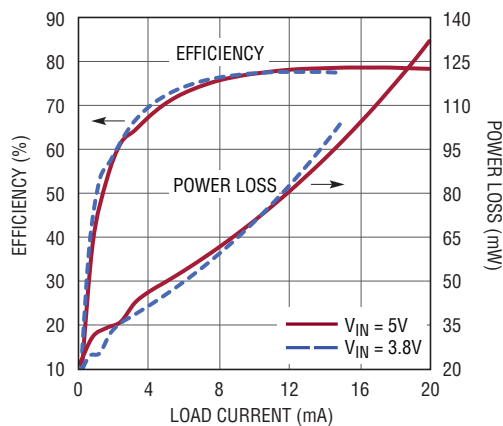
Efficiency and Power Loss (Load Between V_{OUT1} AND V_{OUT2} )
