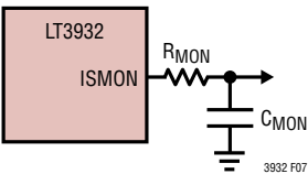
Figure 7. ISMON Filter Configuration
