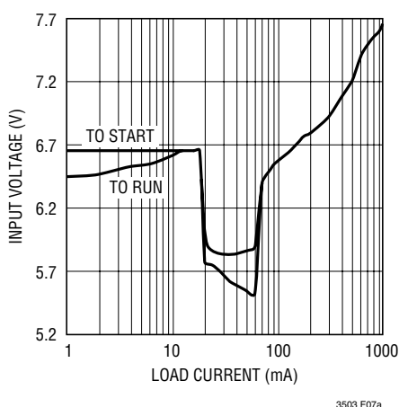
(7a) Typical Minimum Input Voltage, V_{OUT} = 5V
