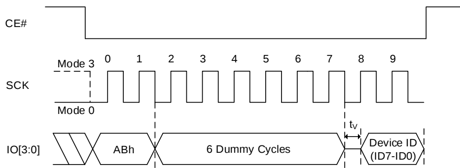
Figure 8.49 Read Product Identification QPI Sequence
