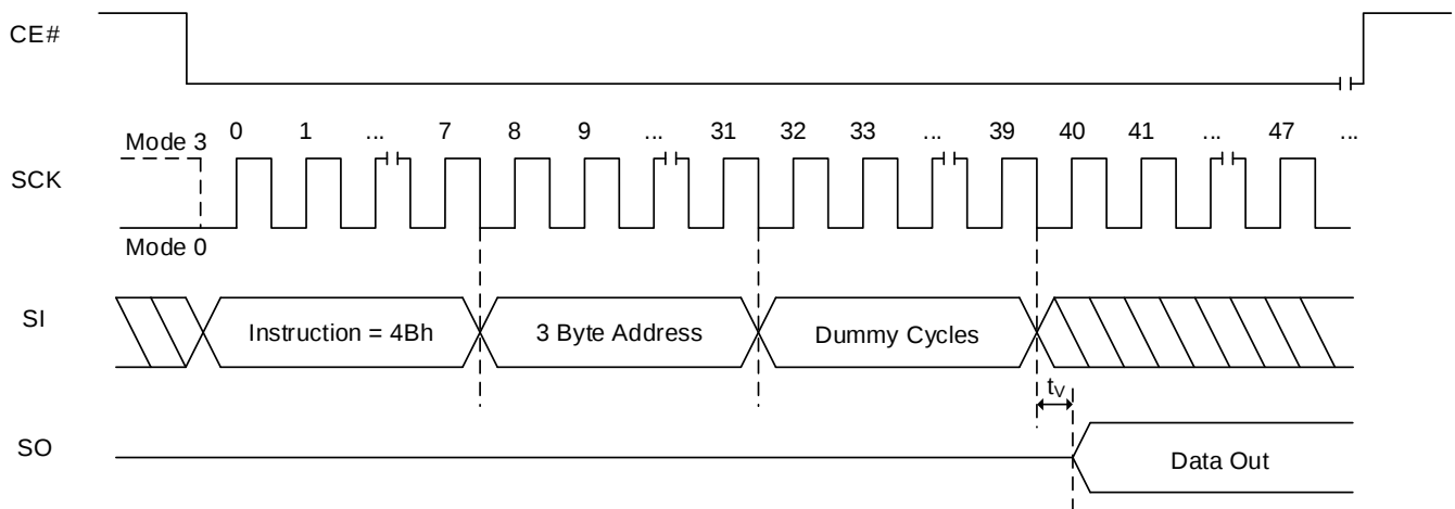
Figure 8.54 RDUID Sequence
