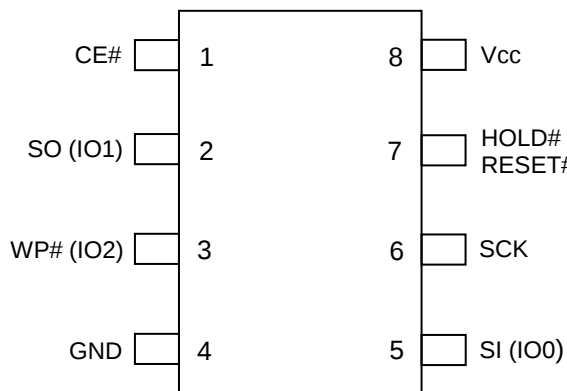
8-pin SOIC 208mil 8-pin SOIC 150mil 8-pin VSOP 208mil 8-pin VVSOP 150mil
