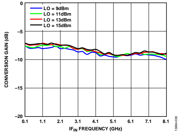
Figure 38. Conversion Gain vs. IF_{IN} Frequency at Various LO Power Levels, T_A = 25^\circ C
