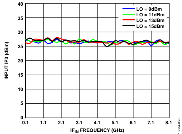
Figure 39. Input IP3 vs. IF_{IN} Frequency at Various LO Power Levels, T_A = 25^\circ C
