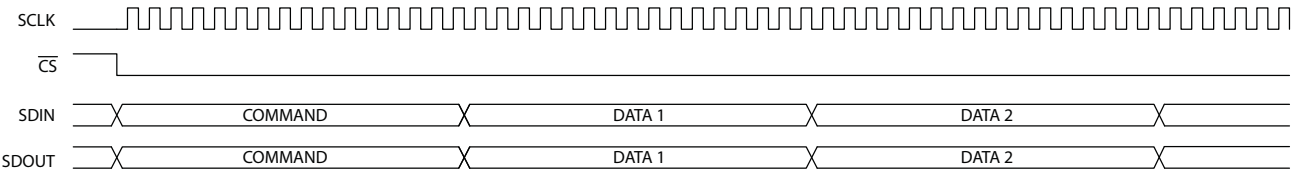
Figure 4-13: GSPI Write Timing – Auto-Increment with Loop-Through Operation (default)
