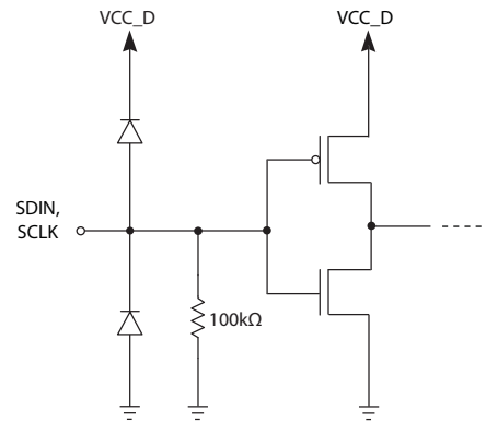
Figure 3-4: SDIN and SCLK
