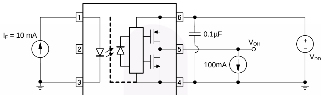
Figure 23. V_{OH} Test Circuit
