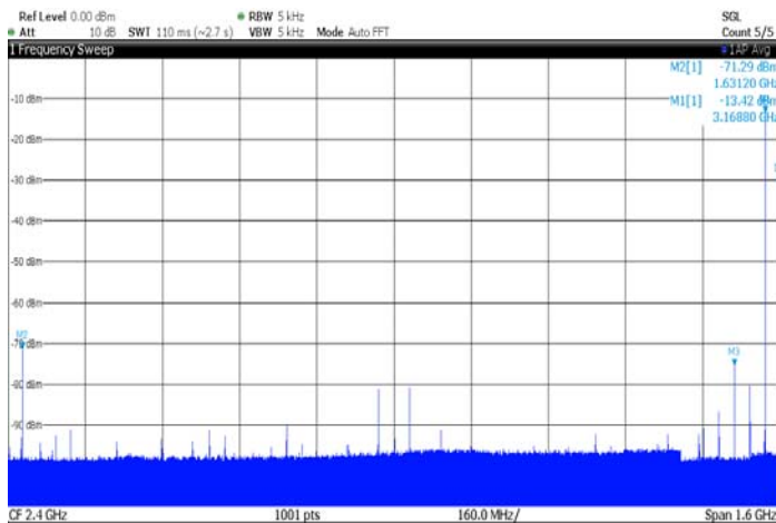
Figure 7-35. Typical SFDR spectrum in RF mode. Fout = 3168 MHz (2 nd Nyquist), MUX2:1, Fs = 3.2 GSps. SFDR = 58 dBc
