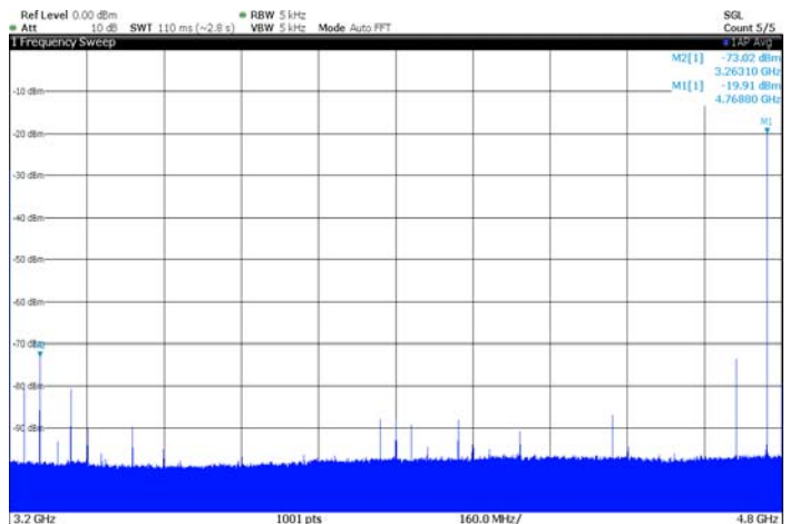
Figure 7-36. Typical SFDR spectrum in RF mode. Fout = 4768 MHz (3 rd Nyquist), MUX2:1, Fs = 3.2 GSps. SFDR = 53 dBc
