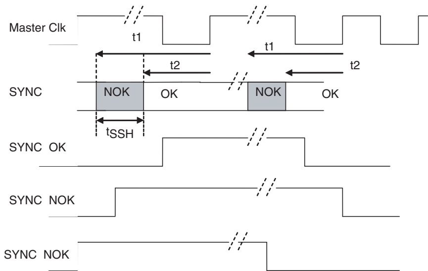
Figure 3-4. SYNC Timing Diagram
