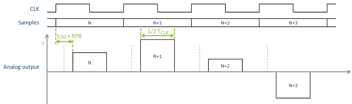
Figure 5-6. RTZ timing diagram
