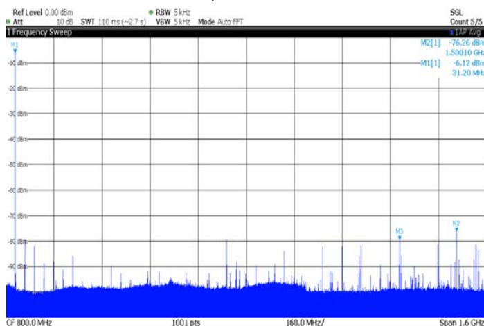
Figure 7-31. Typical SFDR spectrum in NRZ mode. F_{out} = 32 \text{ MHz} (1 st Nyquist), MUX2:1, F_s = 3.2 \text{ GSps} . SFDR = 70 dBc
