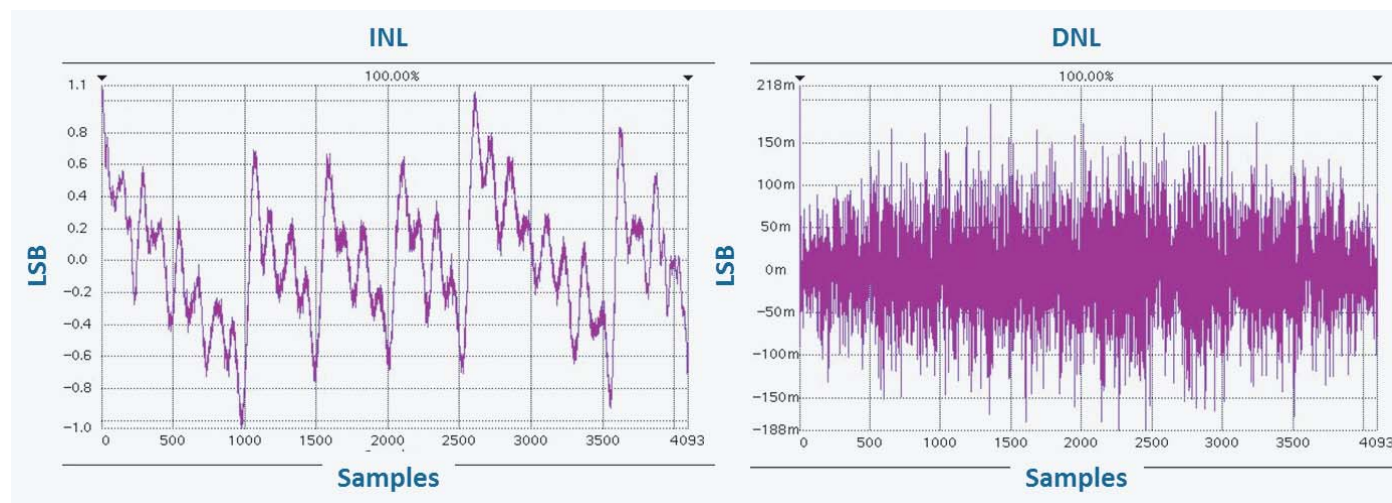
Figure 7-1. INL & DNL measurements at F_{out} = 100\text{ kHz} , F_{clock} = 3\text{ GHz}
