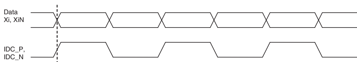
Figure 5-25. IDC timing vs data input:
