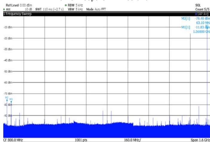
Figure 7-33. Typical SFDR spectrum in NRTZ mode. F_{out} = 1568 \text{ MHz} (1 st Nyquist), MUX2:1, F_s = 3.2 \text{ GSps} . SFDR = 65 dBc
