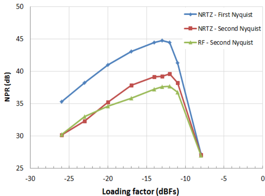
Figure 7-55. NPR versus Loading Factor @ 6.0 Gsps
