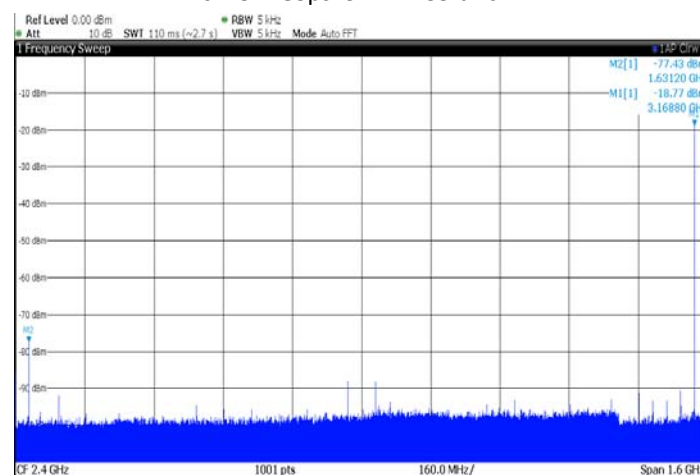
Figure 7-34. Typical SFDR spectrum in RTZ mode. F_{out} = 3168 \text{ MHz} (2 nd Nyquist), MUX2:1, F_s = 3.2 \text{ GSps} . SFDR = 59 dBc
