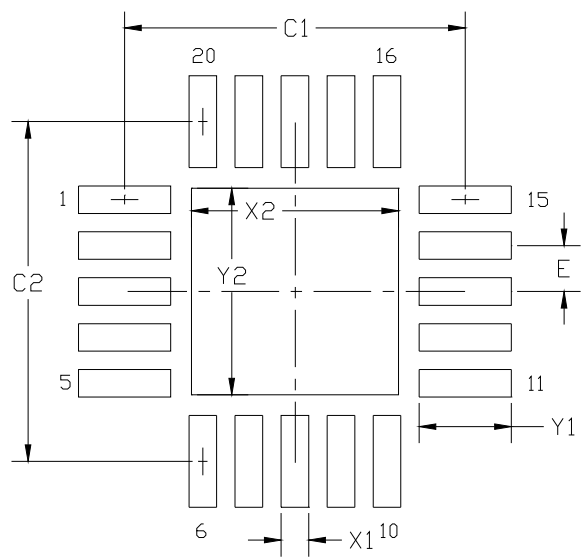
Figure 4.2. QFN-20 Recommended PCB Land Pattern
