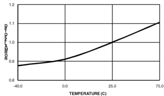
NORMALIZED TPD VS. TEMPERATURE ( V_{CC} = 5.0\text{V} )
