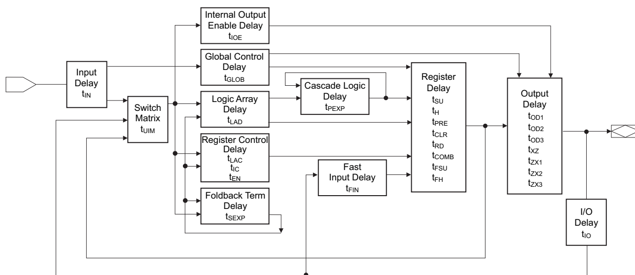
Figure 11-1. Timing Model
