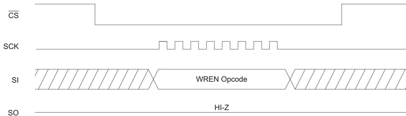
Figure 7-2. WREN Timing
