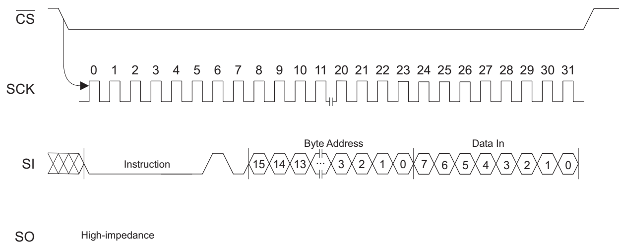
Figure 7-7. Write Timing
