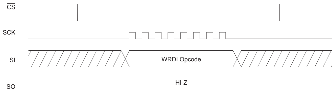
Figure 7-3. WRDI Timing
