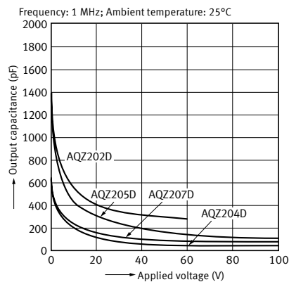
13-2. Output capacitance vs. applied voltage characteristics (AC/DC type)
