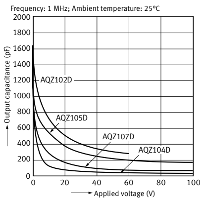
13-1. Output capacitance vs. applied voltage characteristics (DC type)
