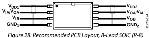
Figure 28. Recommended PCB Layout, 8-Lead SOIC (R-8)
