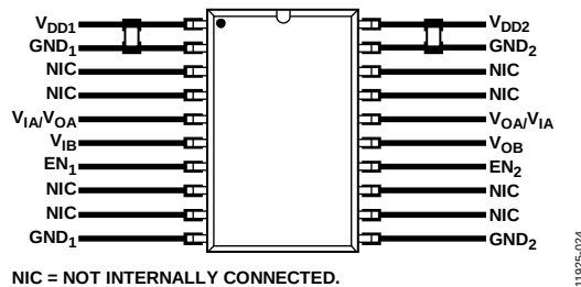
Figure 27. Recommended PCB Layout, 20-Lead SSOP (RS-20)
