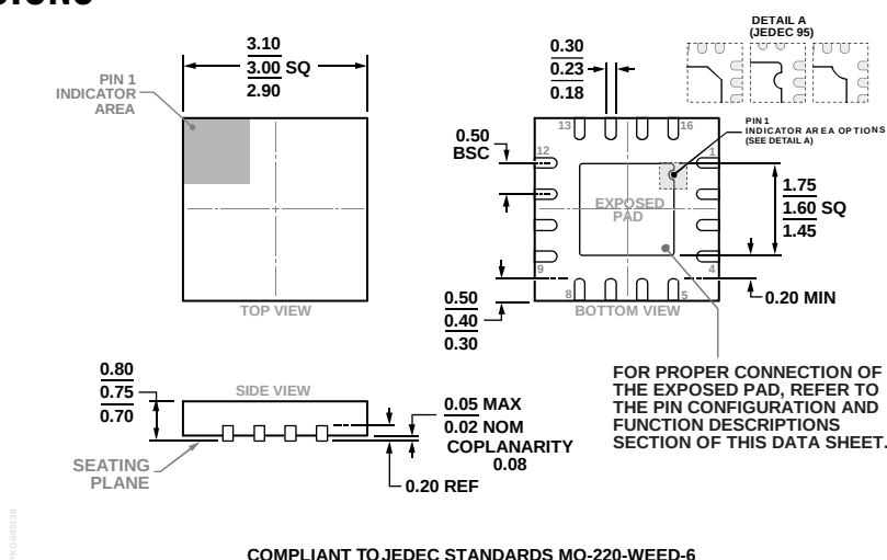
Figure 64. 16-Lead Lead Frame Chip Scale Package [LFCSP] 3 mm × 3 mm Body and 0.75 mm Package Height (CP-16-22) Dimensions shown in millimeters
