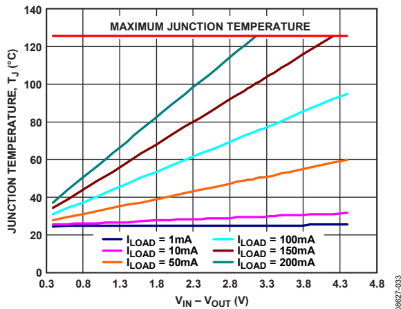
Figure 41. WLCSP 50 mm² of PCB Copper, T_A = 25^\circ\text{C}
