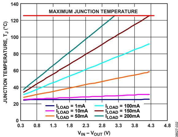
Figure 40. WLCSP 100 mm² of PCB Copper, T_A = 25^\circ\text{C}
