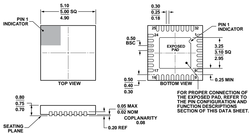
COMPLIANT TO JEDEC STANDARDS MO-220-WHHD. Figure 30. 32-Lead Frame Chip Scale Package [LFCSP_WQ] 5 mm × 5 mm Body, Very Very Thin Quad (CP-32-7) Dimensions shown in millimeters
