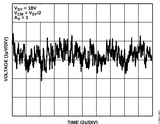
Figure 63. 0.1 Hz to 10 Hz Noise
