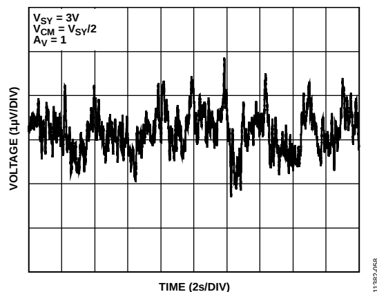
Figure 60. 0.1 Hz to 10 Hz Noise
