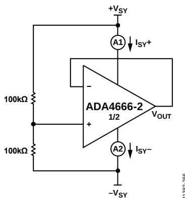
Figure 73. Voltage Follower
