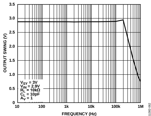
Figure 61. Output Swing vs. Frequency
