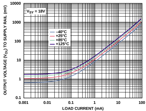
Figure 27. Output Voltage ( V_{OL} ) to Supply Rail vs. Load Current
