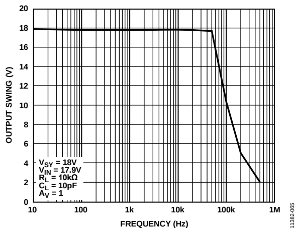
Figure 64. Output Swing vs. Frequency
