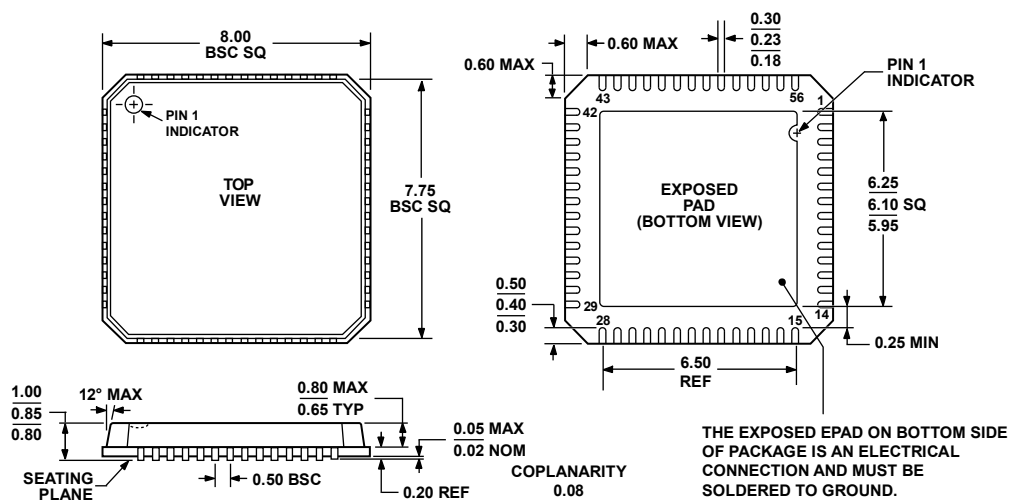
Figure 50. 56-Lead Lead Frame Chip Scale Package [LFCSP_VQ] 8 mm x 8 mm Body, Very Thin Quad (CP-56-1) Dimensions shown in millimeters
