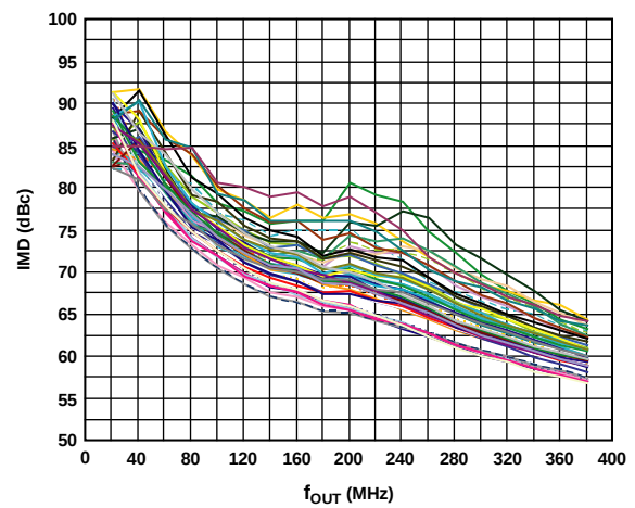
Figure 23. AD9779A Third-Order IMD vs. f_{OUT} , Over 50 Parts, 4× Interpolation, f_{DATA} = 200 MSPS
