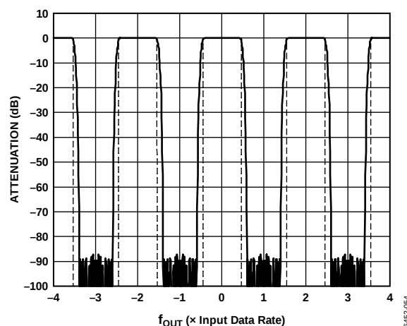
Figure 57. 2× Interpolation, Low-Pass Response to \pm 4\times Input Data Rate (Dotted Lines Indicate 1 dB Roll-Off)
