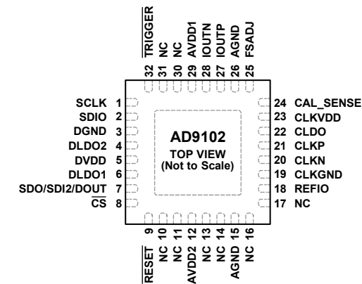
Figure 2. Pin Configuration
