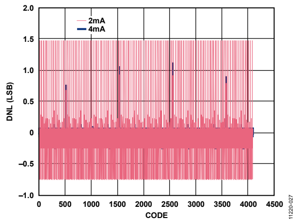
Figure 27. DNL, Two I_{OUTS} Values
