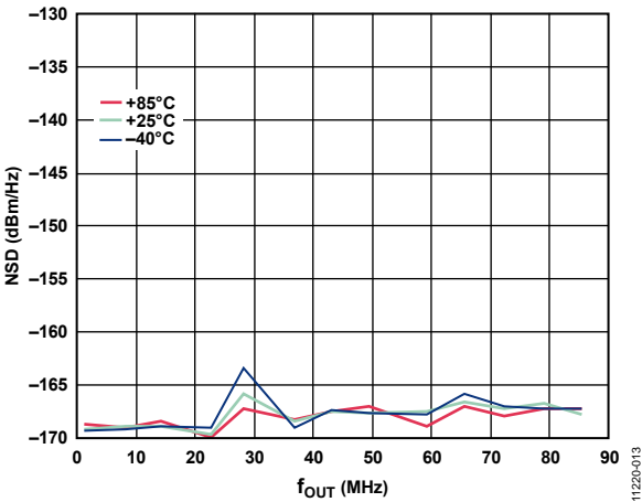
Figure 13. NSD vs. f_{OUT} at Three Temperatures
