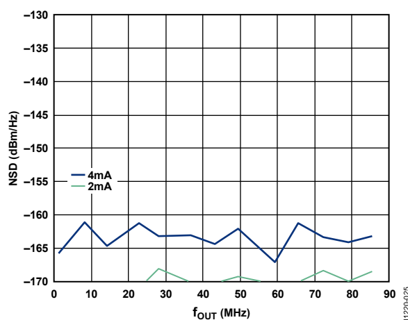
Figure 25. NSD vs. f_{OUT} , Two I_{OUTS} Values
