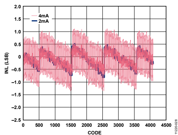
Figure 28. INL, Two I_{OUTS} Values
