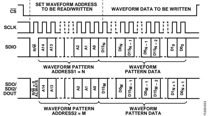
Figure 32. Double SPI Write of SRAM Data
