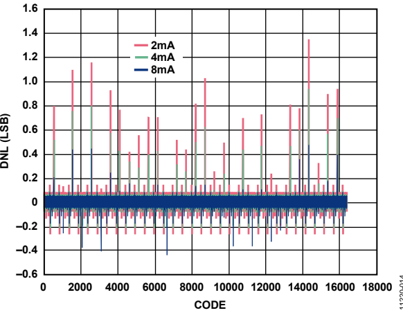
Figure 14. DNL, Three I_{OUTFS} Values
