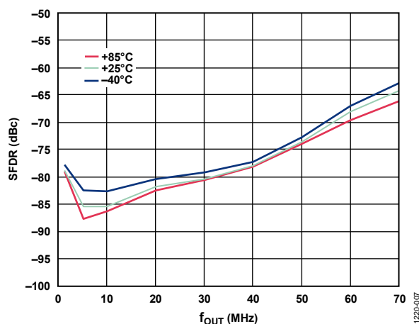
Figure 7. SFDR at Three Temperatures vs. f_{OUT}
