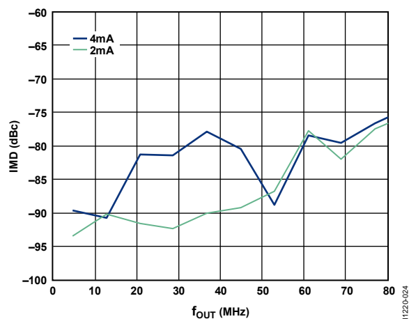
Figure 24. IMD vs. f_{OUT} , Two I_{OUTS} Values
