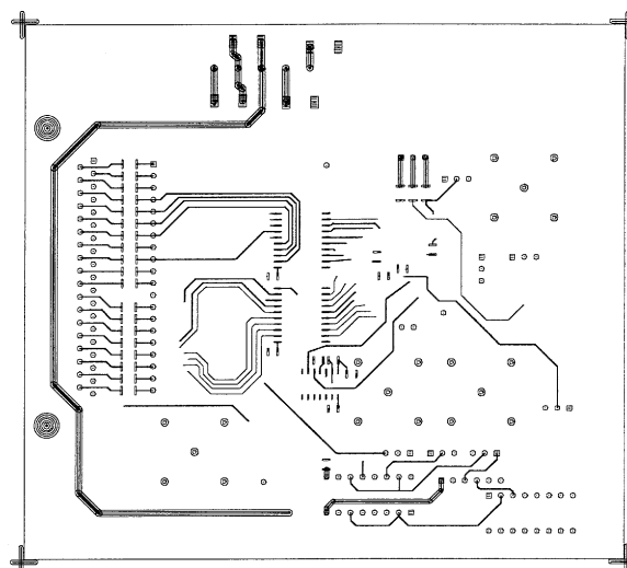
Figure 17. Conductors—Bottom View
