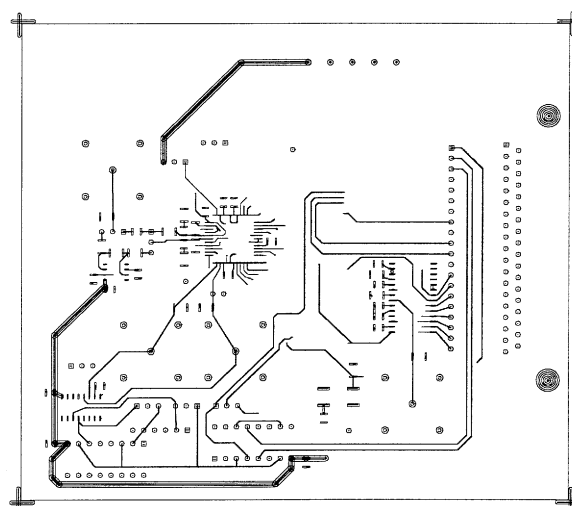
Figure 16. Conductors—Top View
