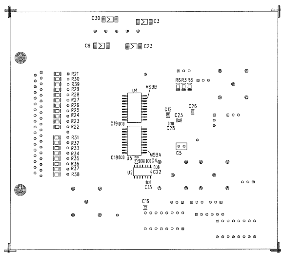
Figure 15. Assembly—Bottom View
