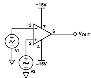
Figure 53. Pulse-Width Modulator
