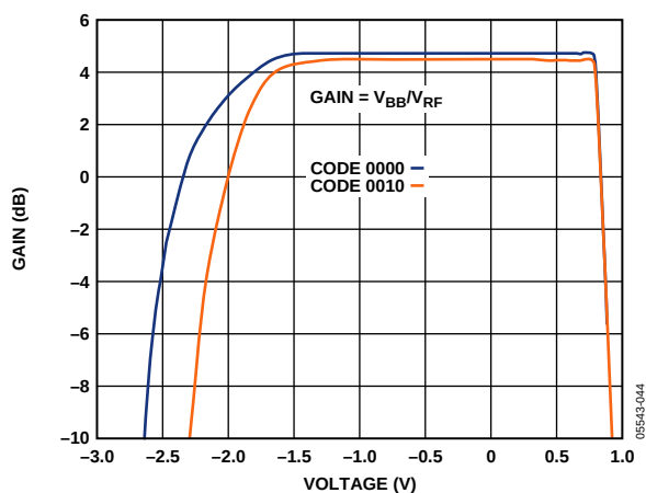
Figure 33. Output Compliance Range (I1PO, Q1PO) (see Figure 50)
