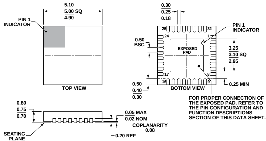
COMPLIANT TO JEDEC STANDARDS MO-220-WHHD. Figure 71. 32-Lead Lead Frame Chip Scale Package [LFCS] 5 mm x 5 mm Body and 0.75 mm Package Height (CP-32-7) Dimensions shown in millimeters
