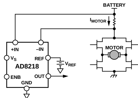
Figure 36. High-Side Current Sensing in Motor Control
