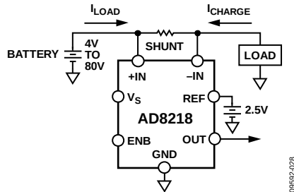
Figure 29. Operation with No V_S Connection
