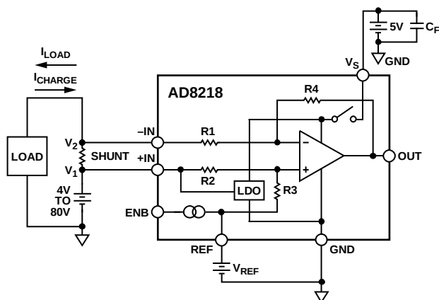
Figure 28. Simplified Schematic
