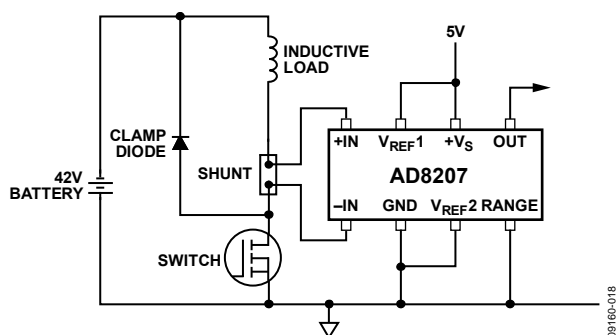
Figure 35. Low-Side Switch
