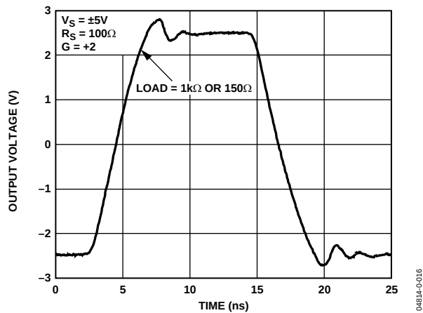
Figure 38. Large Signal Transient Response for Various Loads
