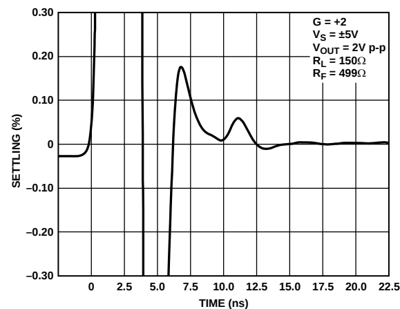
Figure 60. Short Term 0.1% Settling Time
