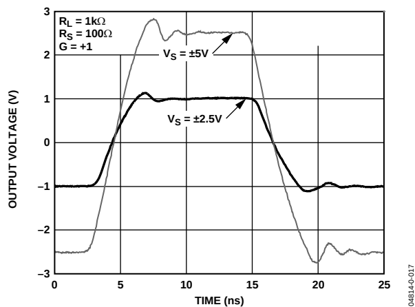
Figure 39. Large Signal Transient Response for Various Supplies
