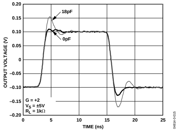
Figure 37. Small Signal Transient Response with Capacitive Load
