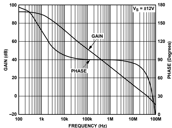
Figure 17. Open-Loop Response
