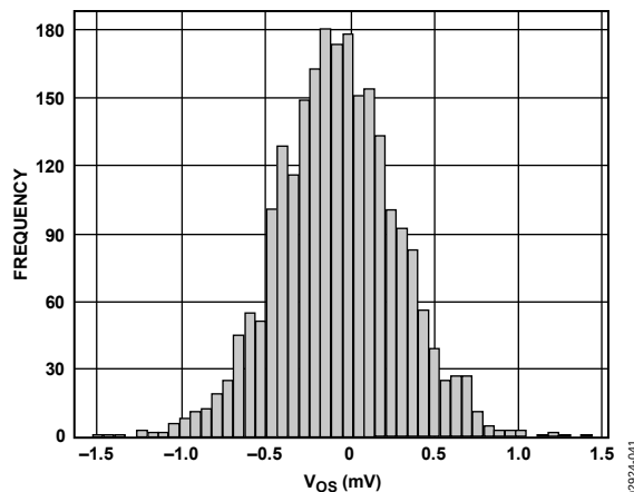
Figure 41. Initial Offset
