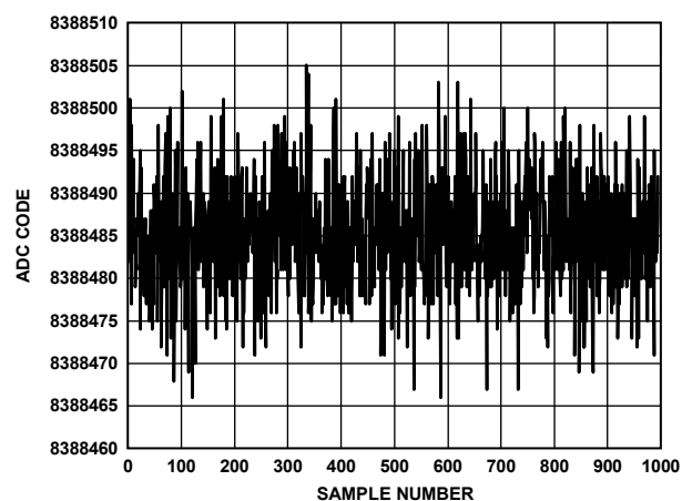
Figure 6. Noise (Analog Input Buffers Disabled, V_{REF} = 5\text{ V} , Output Data Rate = 2.6 kSPS)
