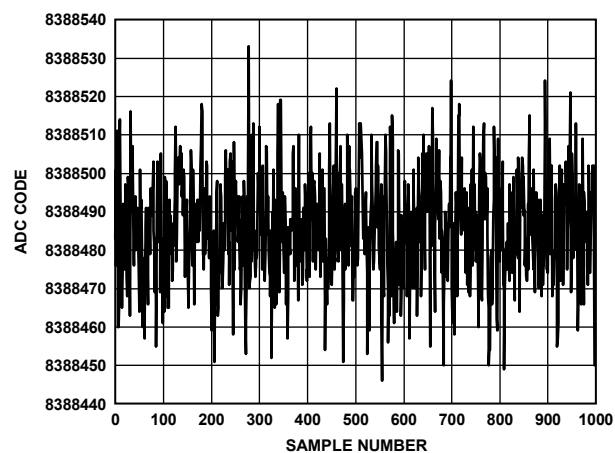
Figure 7. Noise (Analog Input Buffers Disabled, V_{REF} = 5\text{ V} , Output Data Rate = 31.25 kSPS)
