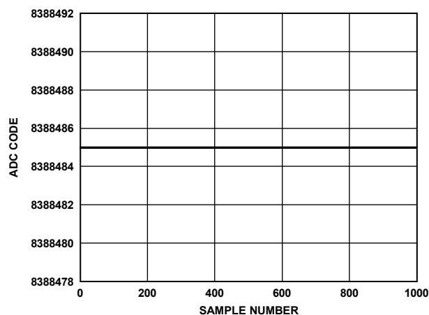
Figure 5. Noise (Analog Input Buffers Disabled, V_{REF} = 5\text{ V} , Output Data Rate = 1.25 SPS)
