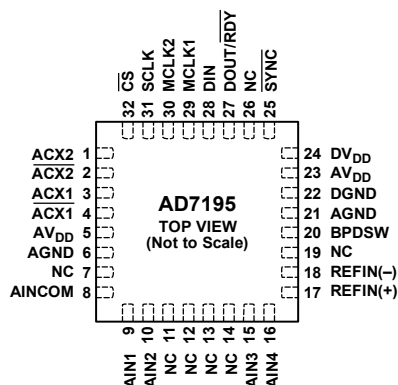
Figure 5. Pin Configuration
