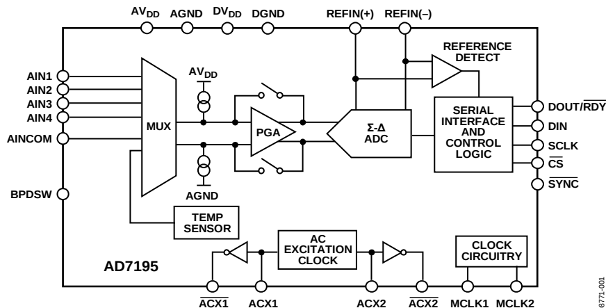
Figure 18. Block Diagram
