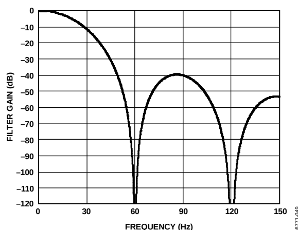
Figure 37. Sinc 3 Filter Response ( FS[9:0] = 80 )
