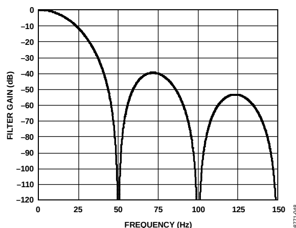
Figure 36. Sinc 3 Filter Response ( FS[9:0] = 96 )
