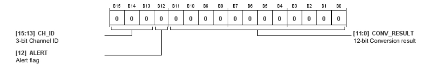
Figure 47. Conversion Result Register
