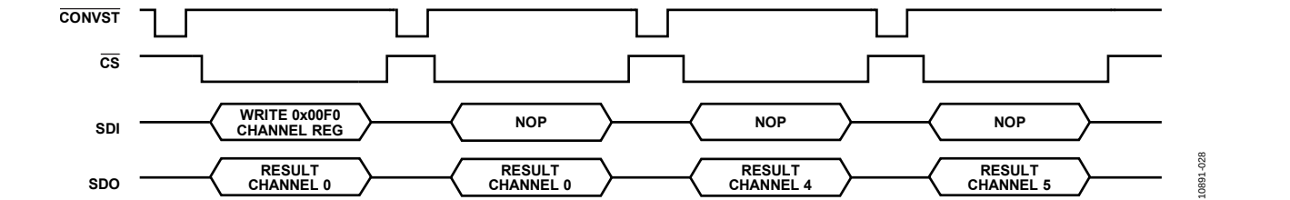
Figure 55. Channel Sequencer
