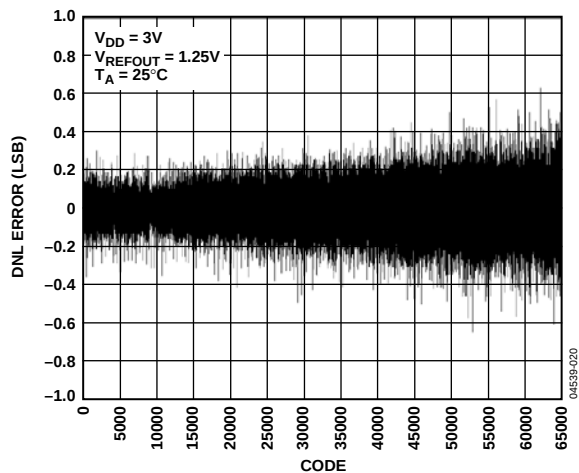
Figure 15. DNL—AD5660-1
