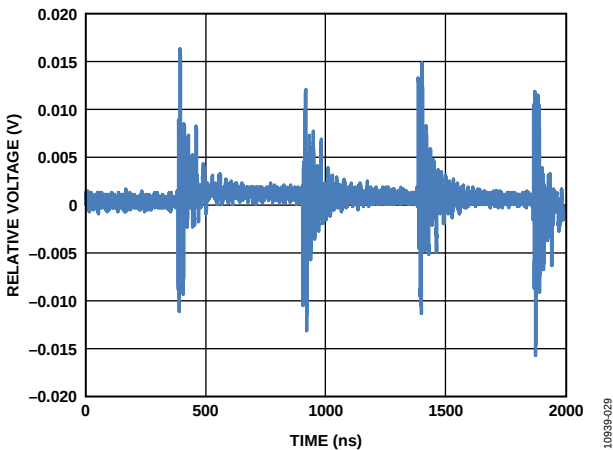
Figure 30. Digital Feedthrough
