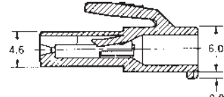
Section X-X
