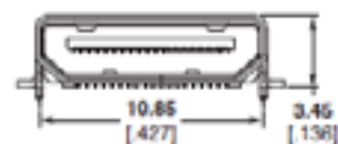
HDMI-C Connector
