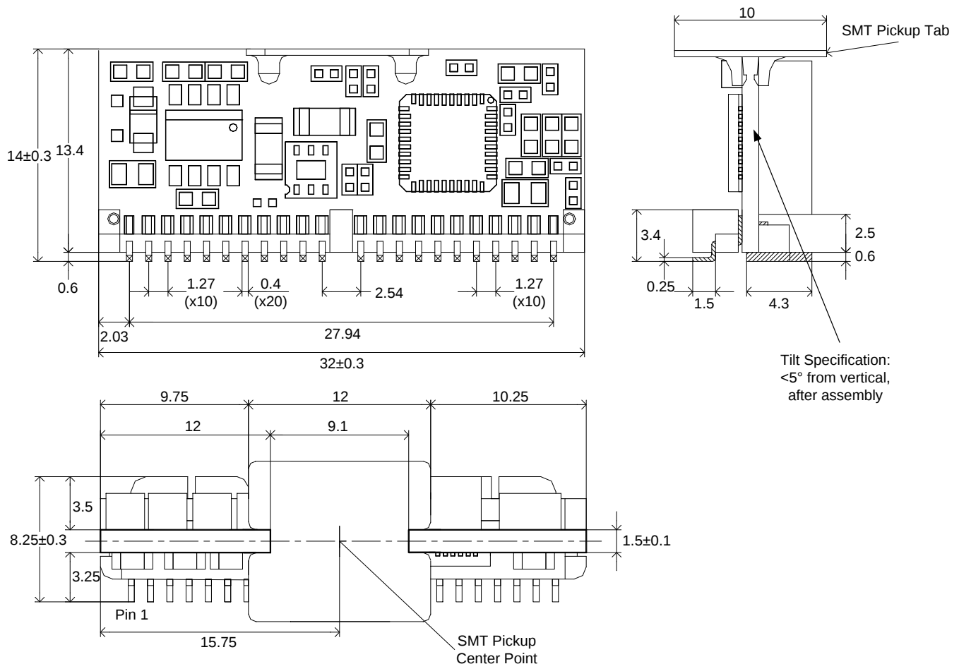
Figure 58. Mechanical Drawing
