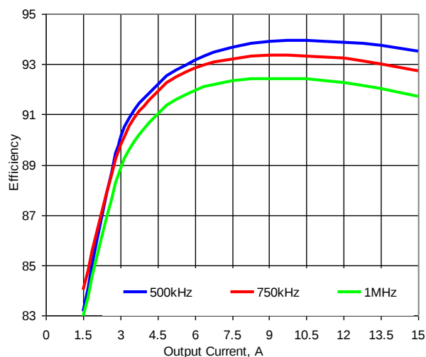
Figure 9. Efficiency vs. Load. V_{in}=12V , V_{out}=5V
