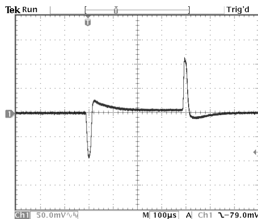
Figure 22. Vin=3V, Vout=1V. Bandwidth is 30kHz
