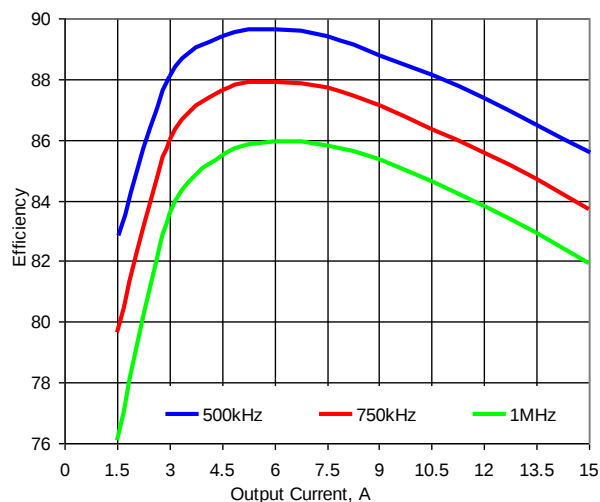
Figure 8. Efficiency vs. Load. V_{in}=5V , V_{out}=1.2V
