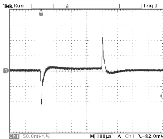
Figure 21. Vin=5V, Vout=2.5V. Bandwidth is 40kHz
