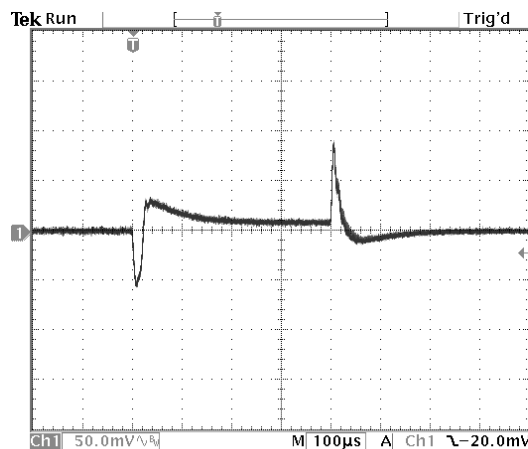
Figure 20. Vin=5V, Vout=1V. Bandwidth is 40kHz
