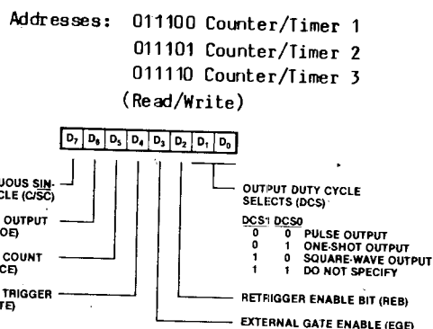
Figure 2-15. Counter/Timer Mode Specification Registers
