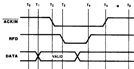
Figure 3-4. Strobed Input Handshake Timing Diagram
