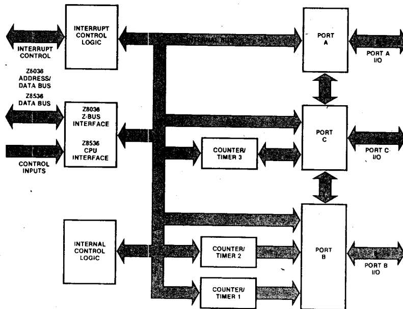
Figure 1-1. Z8036/Z8536 Z-C10/C10 Block Diagram
