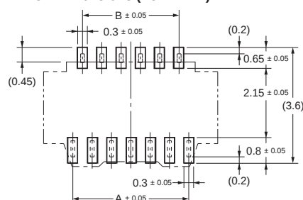
Applicable FPC Dimensions
