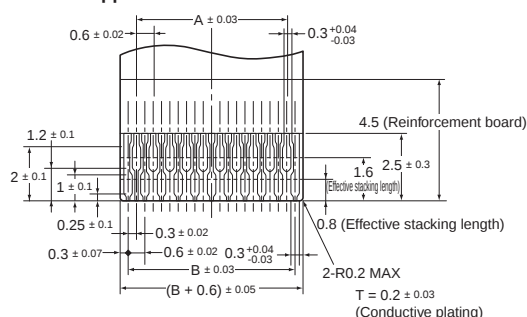
Applicable FPC Dimensions
