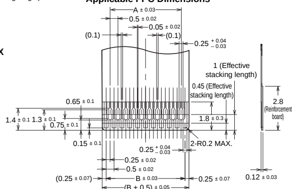
Applicable FPC Dimensions
