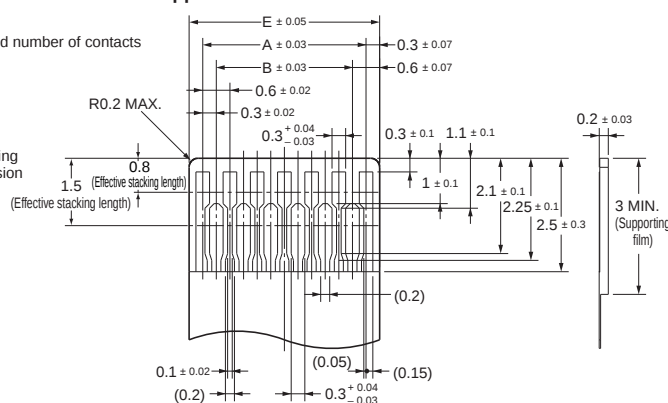
Applicable FPC Dimensions
