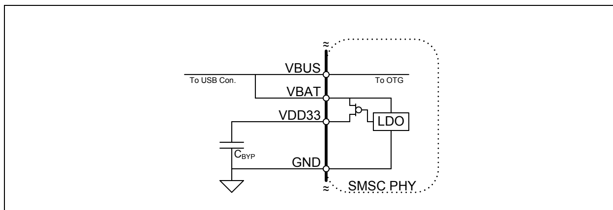
Figure 5.5 Powering the USB3317 from the USB Cable Vbus
