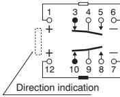
Schematic (Bottom view) 2 coil latching (L2)
