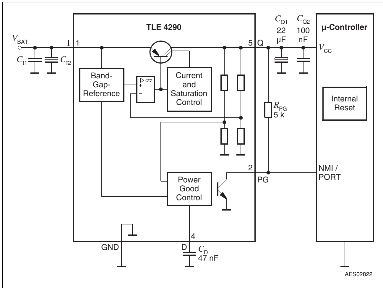
Figure 4 Application Diagram
