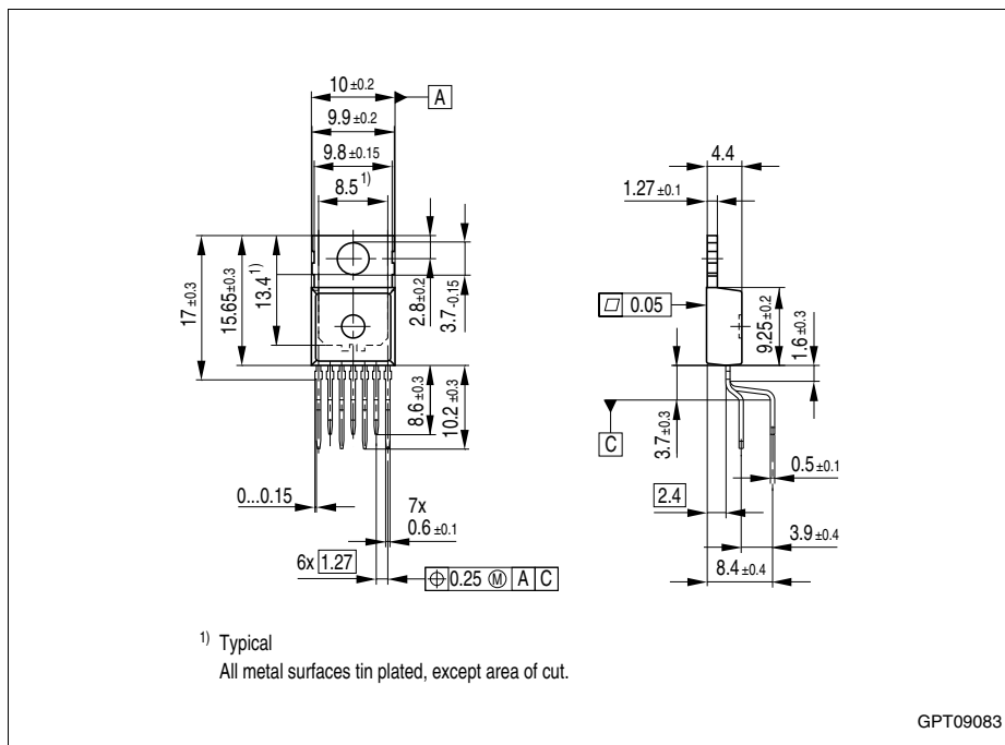
Figure 8 PG-TO220-7-11 (Plastic Transistor Single Outline)
