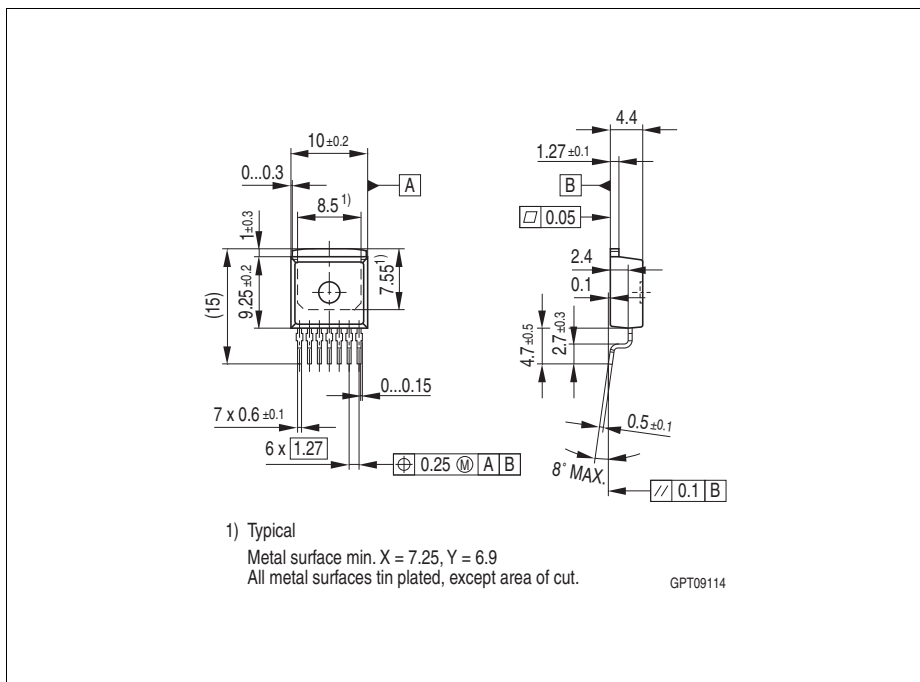
Figure 9 PG-TO263-7-1 (Plastic Transistor Single Outline)
