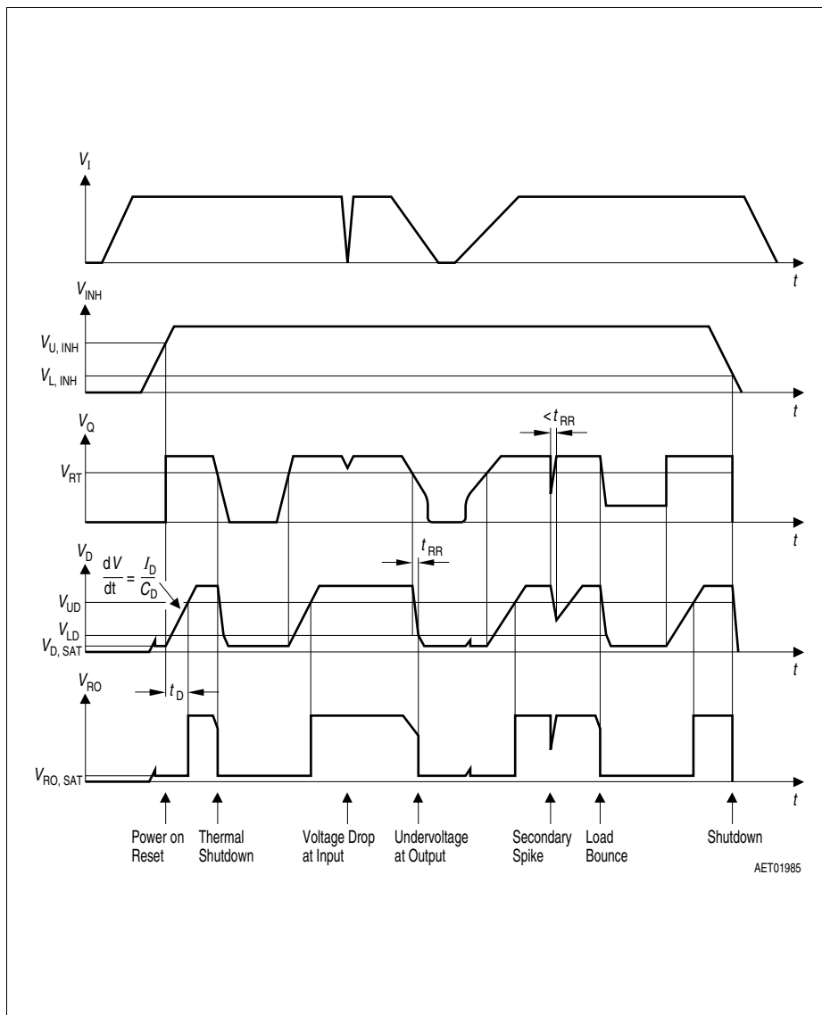
Figure 6 Time Response
