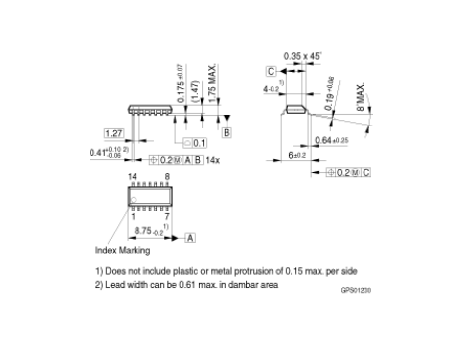
Figure 11 PG-DSO-14-30 (Plastic Dual Small Outline)
