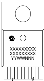
5-Lead TO-220
