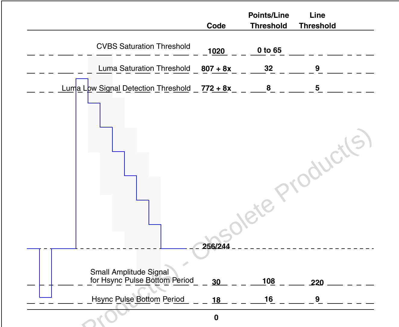
Figure 9: AGC Flowchart
