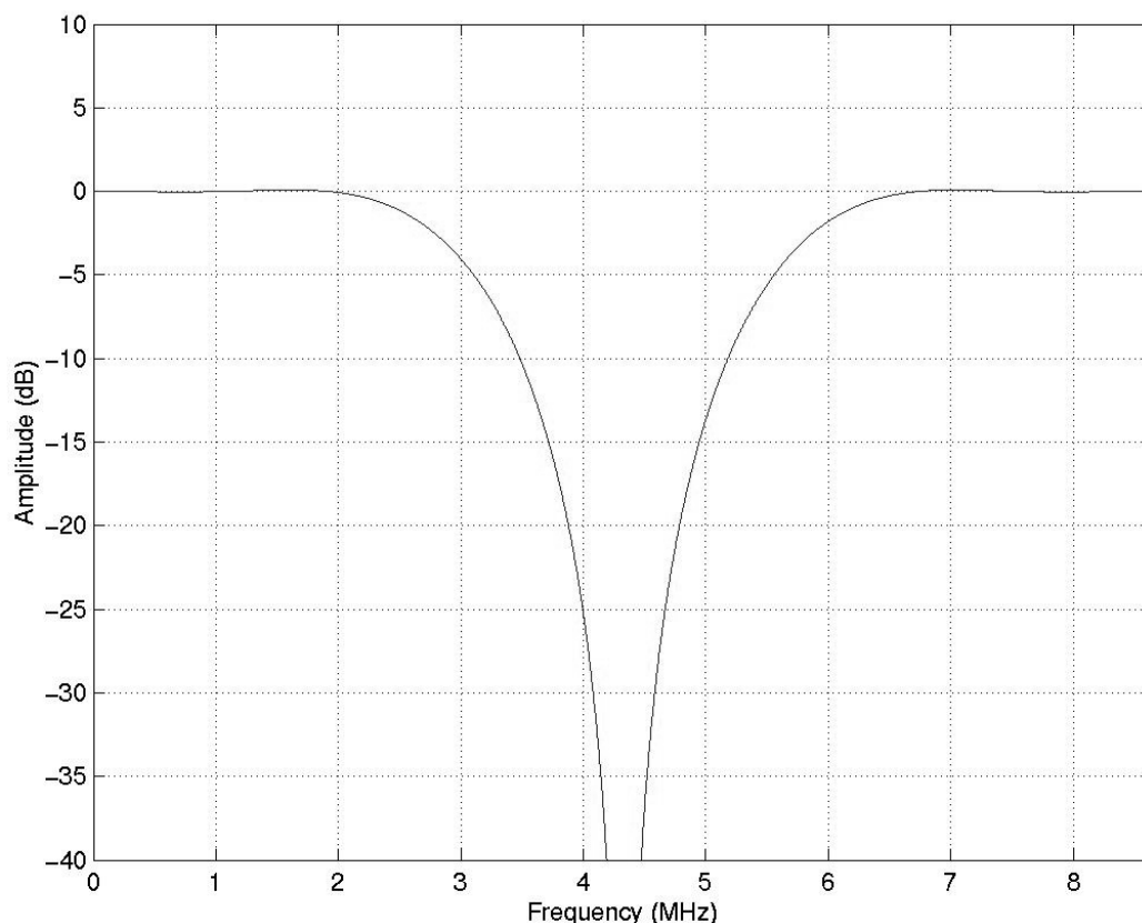
Figure 10: SECAM Trap Filter Frequency Response
