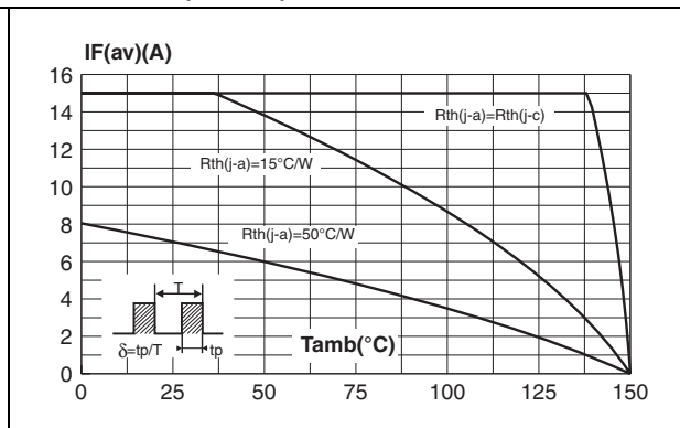
Figure 3. Average forward current per diode versus ambient temperature (δ = 0.5)
